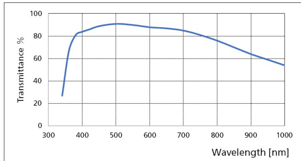
Plan Achromat Phase 40x / Plan Fluor 40x
